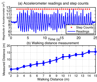
Fig. 12. (a) Step counter readings and (b) measurement accuracy versus walking distances.
